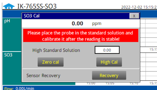
Figure. 18 - SO3 Calibration
