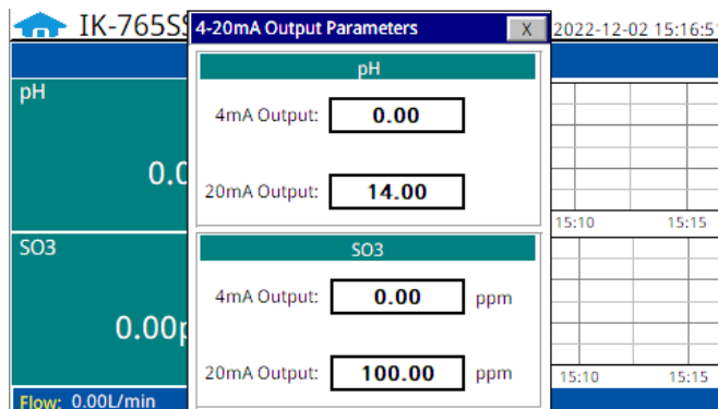
Figure. 12 - 4-20mA Output Setting
