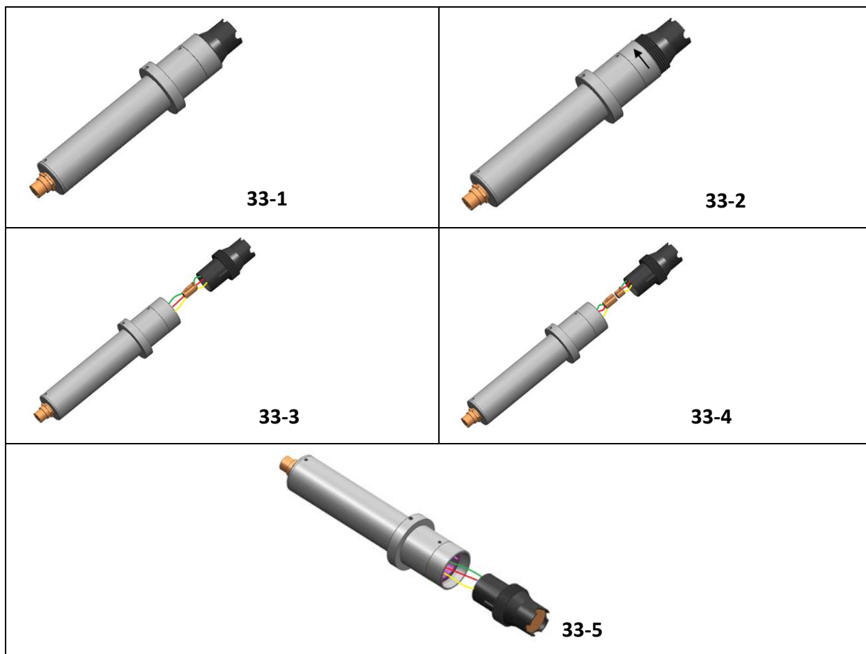
Figure 33 - Replacing EH-765 pH and Sulfite Electrode Head
