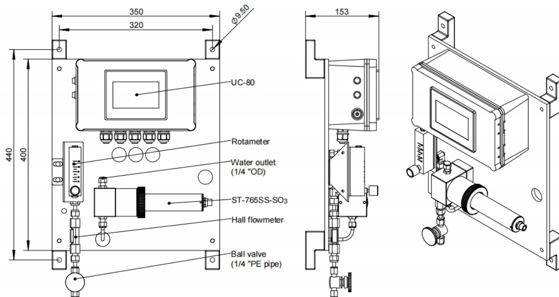
Figure. 1 - IK-765SS-SO3 controller size and installation size
