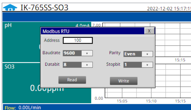
Figure. 13 - Modbus RTU
