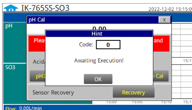
Figure. 17 - pH Calibration Success Prompt
